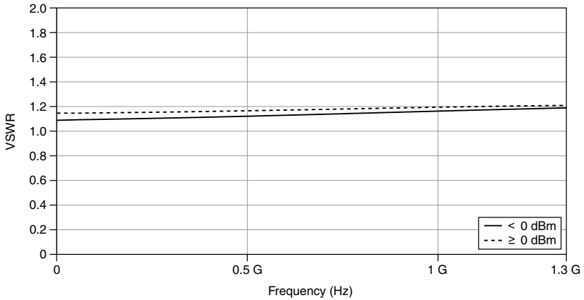
Figure 6. Measured VSWR
