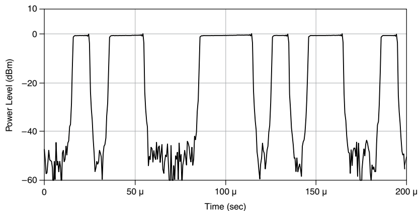
Figure 8. OOK Diagram, 1.0 GHz Carrier, 100 kHz Symbol Rate, Ninth-Order PRBS
