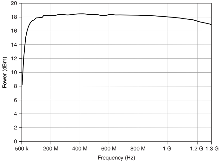
Figure 4. Measured Maximum Available Power
