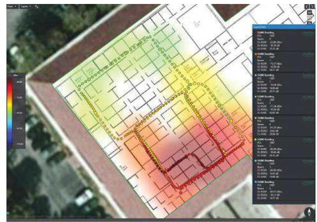
3D Indoor Maps with Base Station Data are Generated by the NEON Signal Mapper
