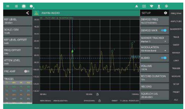
AM/FM Demod
