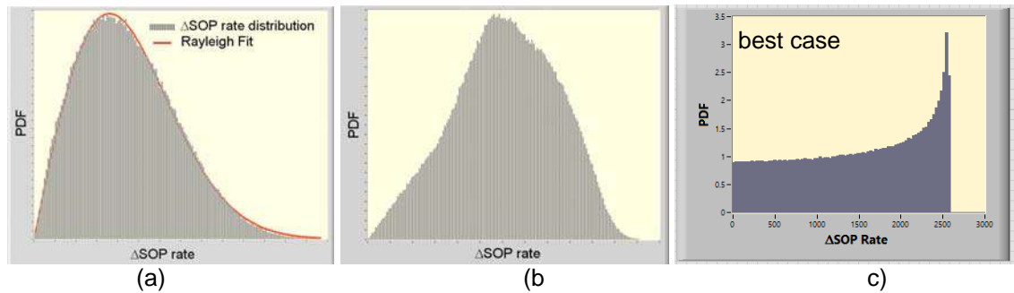
Figure 2. SOP variation rate distributions for (a) Rayleigh, (b) Triangle, and (c) Tornado scrambling methods. The Tornado distribution is input polarization dependent. The figure shows the best case.
