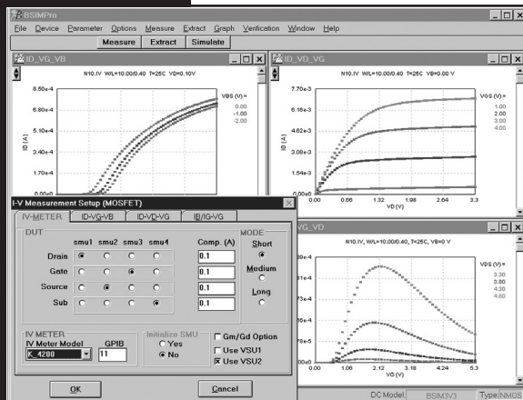
Cadence provides a 4200-SCS driver for BSIMProPLUS.
